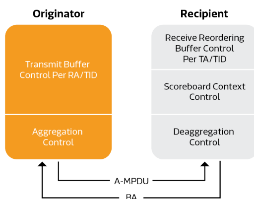
Figure 1. HT-Immediate BA Architecture
