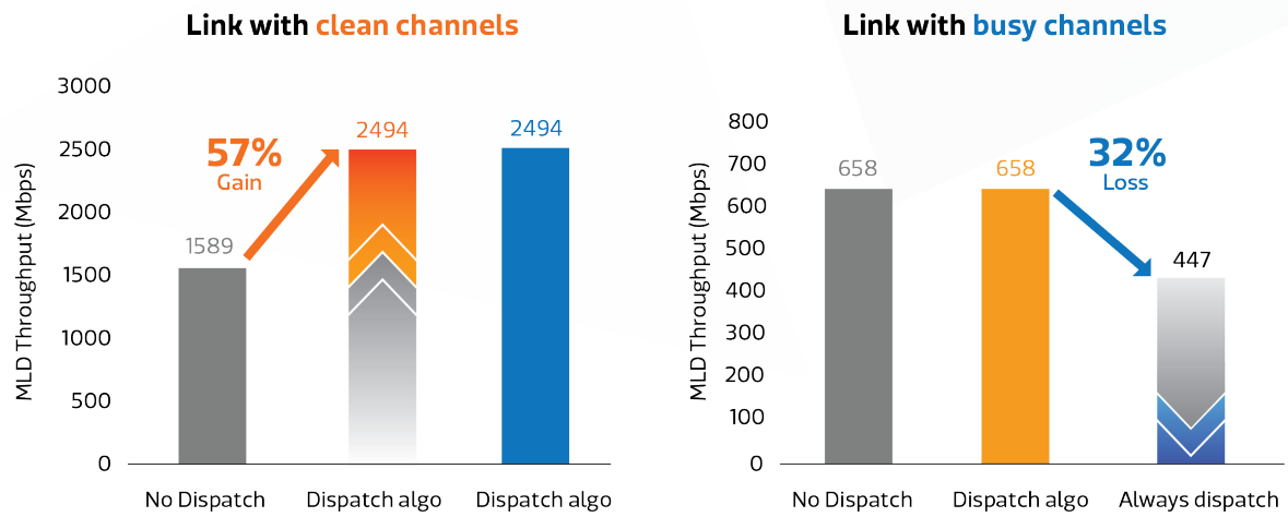
Figure 6. Comparisons of Throughput Efficiency
