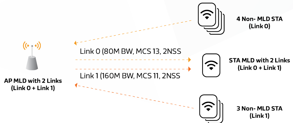
Figure 5. Network Topology of Link with Busy Channels
