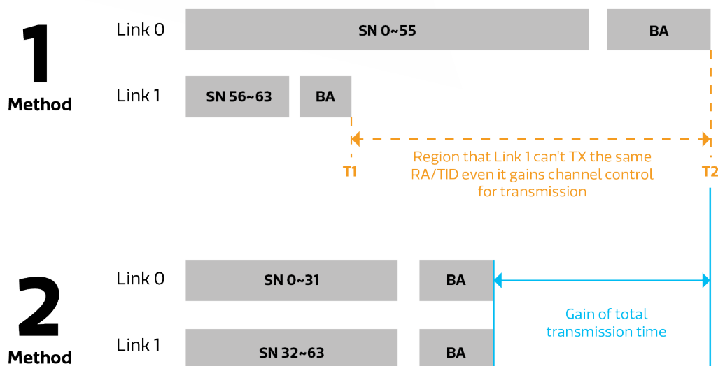
Figure 2. Examples of Methods for Dispatching MPDUs over Two Links
